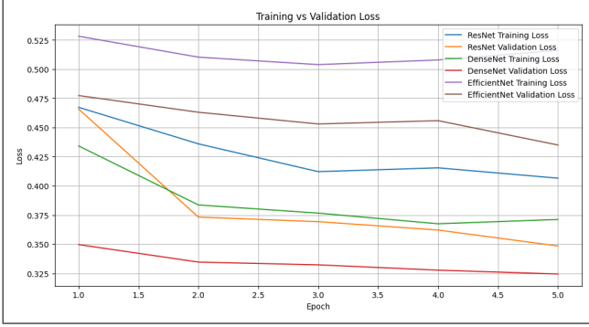
Figure 2. Training and Validation Loss Curves
